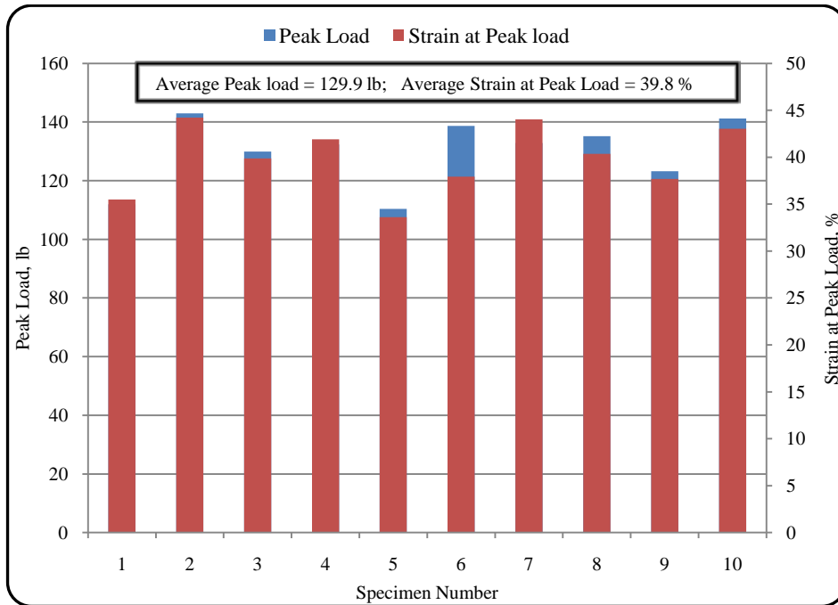
Figure 17 Peak Loads and corresponding strains for dry, machine direction (DMD) on BSRF
