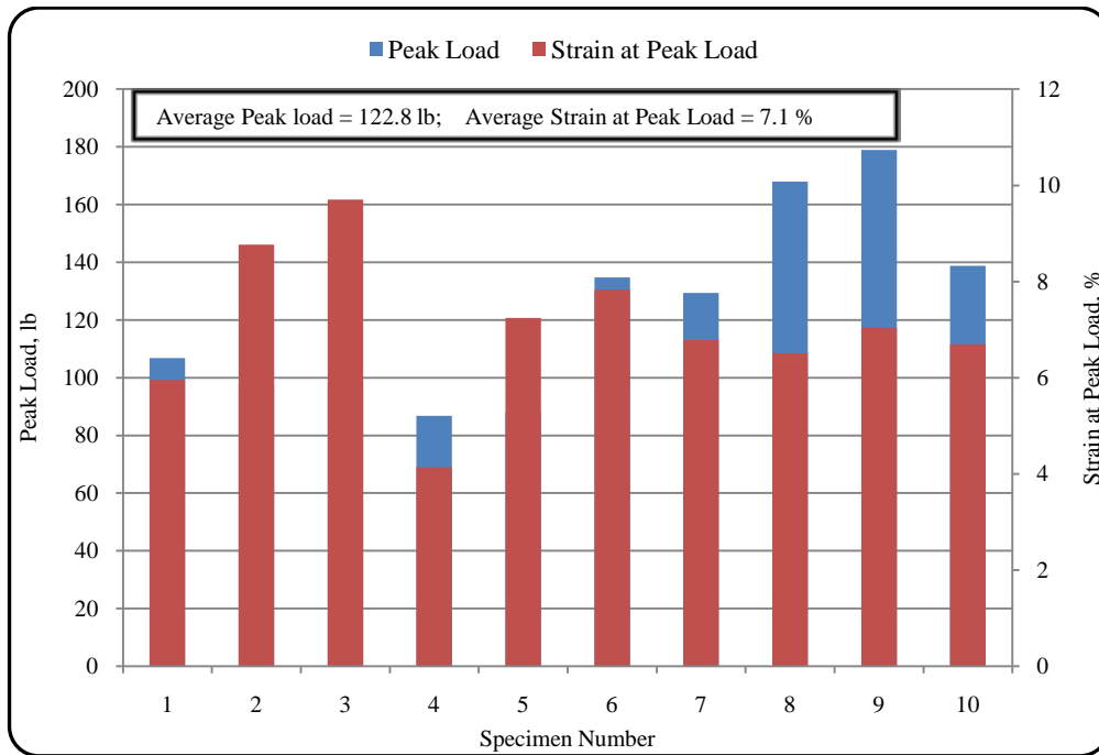
Figure 27 Peak loads and corresponding strains for WCMD on Type III silt fence
