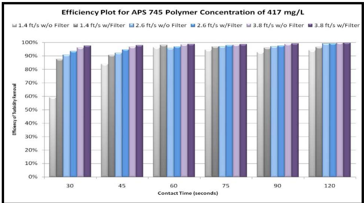
Figure 53 Plot of efficiencies for polymer APS 745 at a concentration of 417 mg/L
