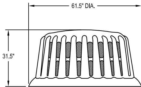
ELEVATION VIEW
