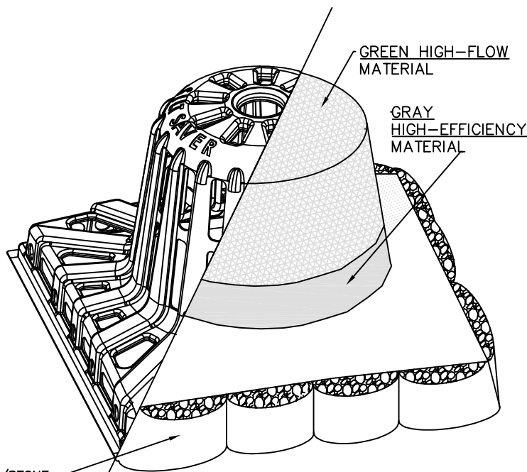
ISOMETRIC ASSEMBLY VIEW OF A1100A-DOT
